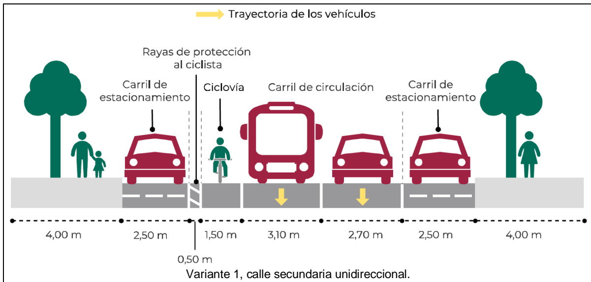
Figura 68.- Calles colectoras [1] [2] [3]
