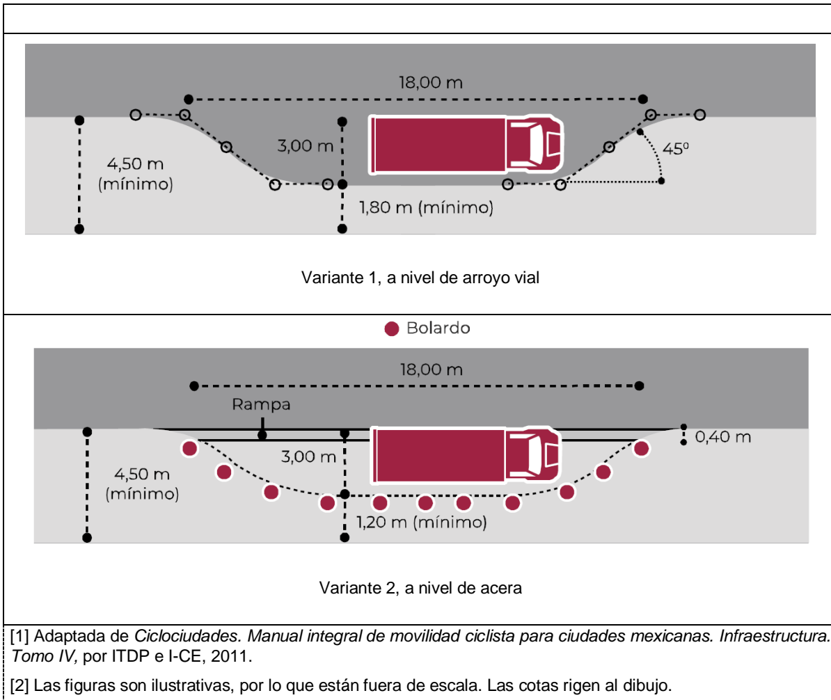
Figura 76.- Bahías [1] [2]
